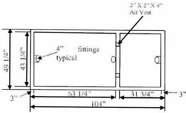
Section A
